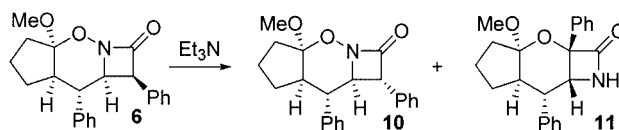
Scheme 5. Base-initiated rearrangement of N -organyloxy \beta -lactam
