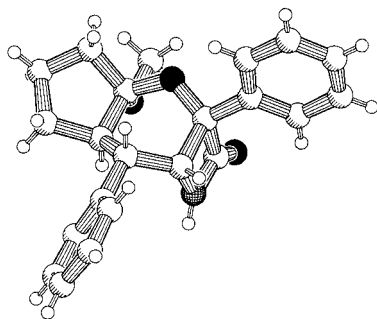
Figure 2. X-ray structure of lactam 11 [6]
