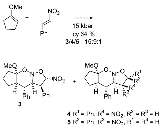
Scheme 3. (4+2)/(3+2) cycloaddition of \beta -nitrostyrene and 1-methoxycyclopent-1-ene
