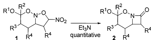
Scheme 1. Rearrangement to give N -organyloxy \beta -lactams
