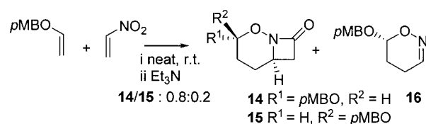
Scheme 6. Synthesis of N -organyloxy \beta -lactam 14 and 15
