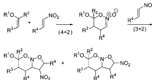
Scheme 2. Formation of nitroso acetals
