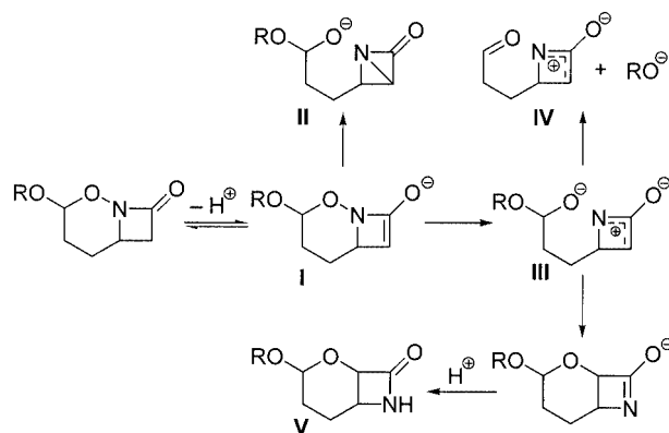
Scheme 7. Proposed mechanism for rearrangement of N -organyloxy \beta -lactam
