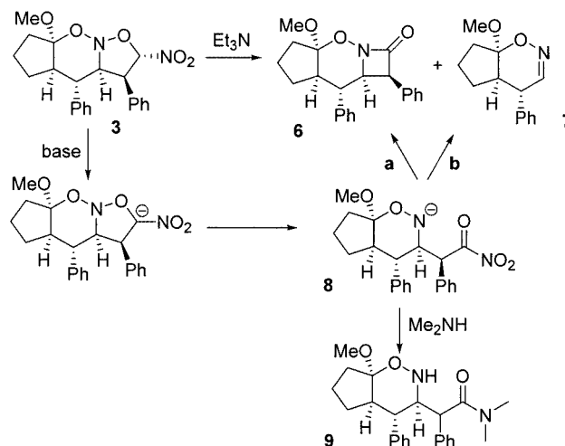
Scheme 4. Formation of N -organyloxy \beta -lactam 6 and trapping of intermediate 8
