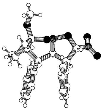
Figure 1. X-ray structure of nitroso acetal 3 [6]
